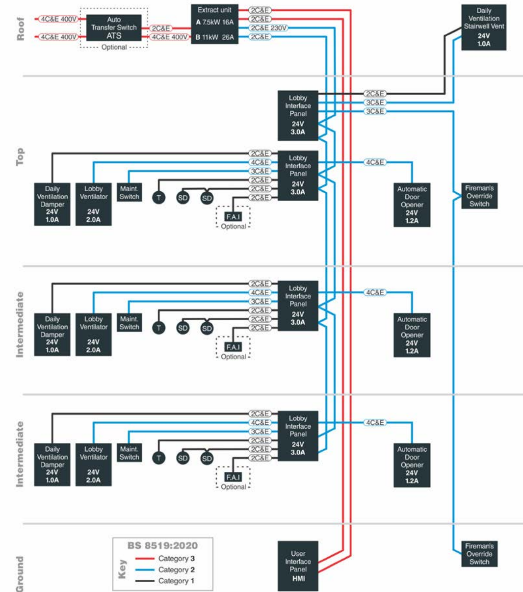
UniForce Single Line Diagram with Daily Ventilation
