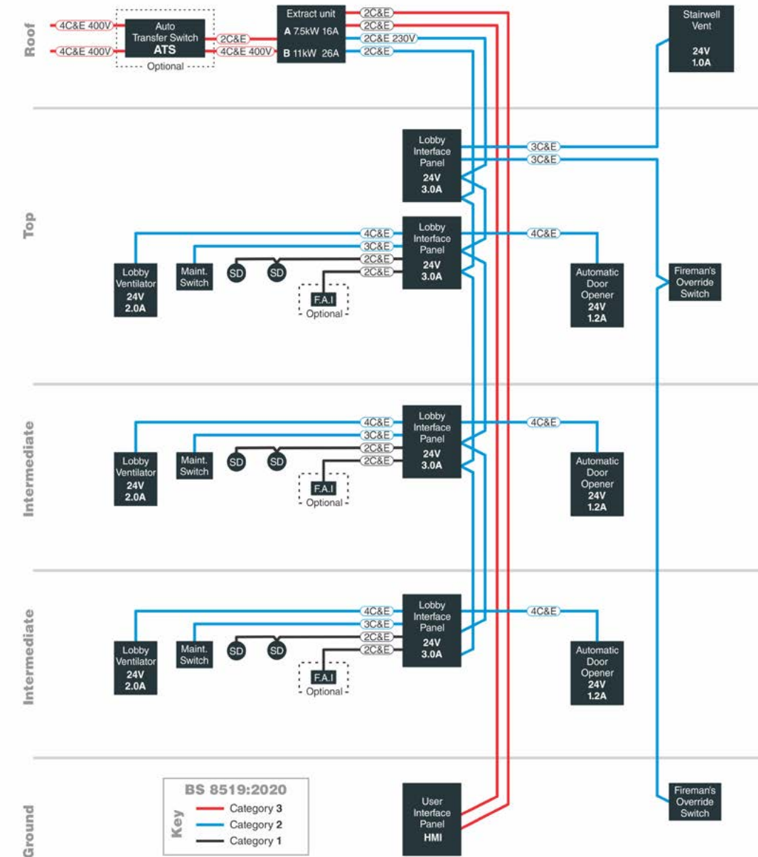
UniForce Single Line Diagram
